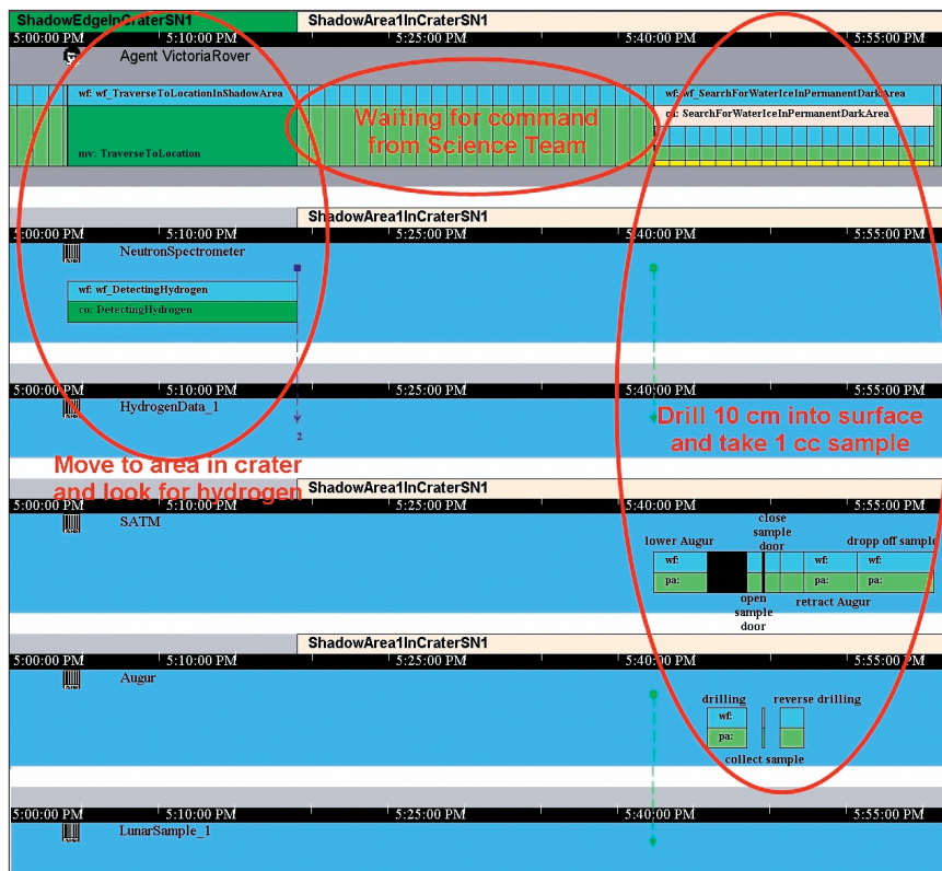
Figure 7. Victoria rover scenario activities.
