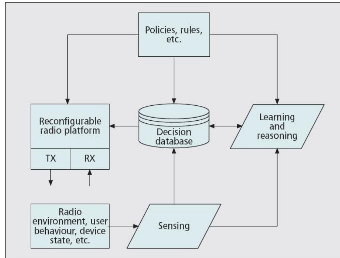
■ Figure 3. Cognitive radio functionality.
