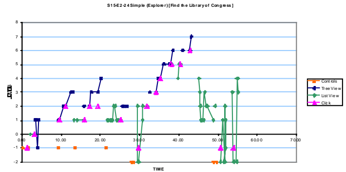
Figure 11. Scent-finding and scent-following on the Explorer for the Library of Congress task.
