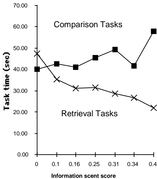
Figure 4. Performance times in Experiment 1 as a function of question type and information scent.
